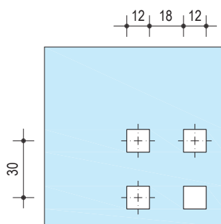
Unity 3 U3 (foratura quadrata) 3.5x3.5
