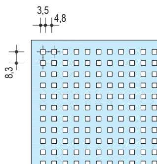
Unity 3 U3 (foratura quadrata) 3.5x3.5
